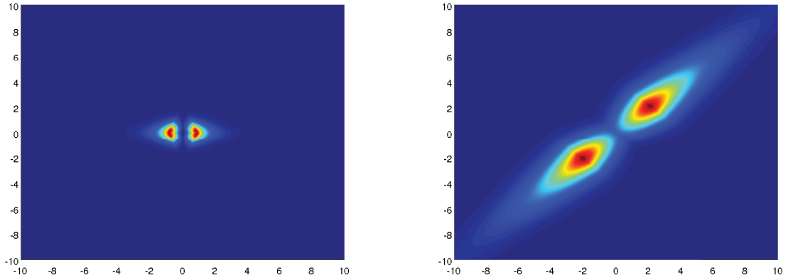
Figure 1. Left: The weight function \min\left(1, s_\lambda^{-1} + |\xi_1| + s_\lambda^{-(1-\alpha)} |\xi_2|\right)^M \langle |\xi| \rangle^{-N_1} \langle \xi_2 \rangle^{-N_2} for s_\lambda = 8 , M = 3 , N_1 = N_2 = 2 . Right: Approximate frequency support of a corresponding \frac{1}{2} -molecule \hat{m}_\lambda with \theta_\lambda = \pi/4 .
