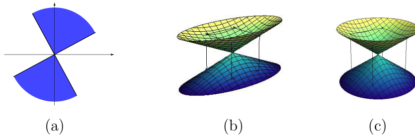
Figure 1: (a) shows a sample region of vectors of a non-scalable frame in \mathbb{R}^2 . (b) and (c) show examples of sets in \mathcal{C}_3 which determine sample regions in \mathbb{R}^3 .
