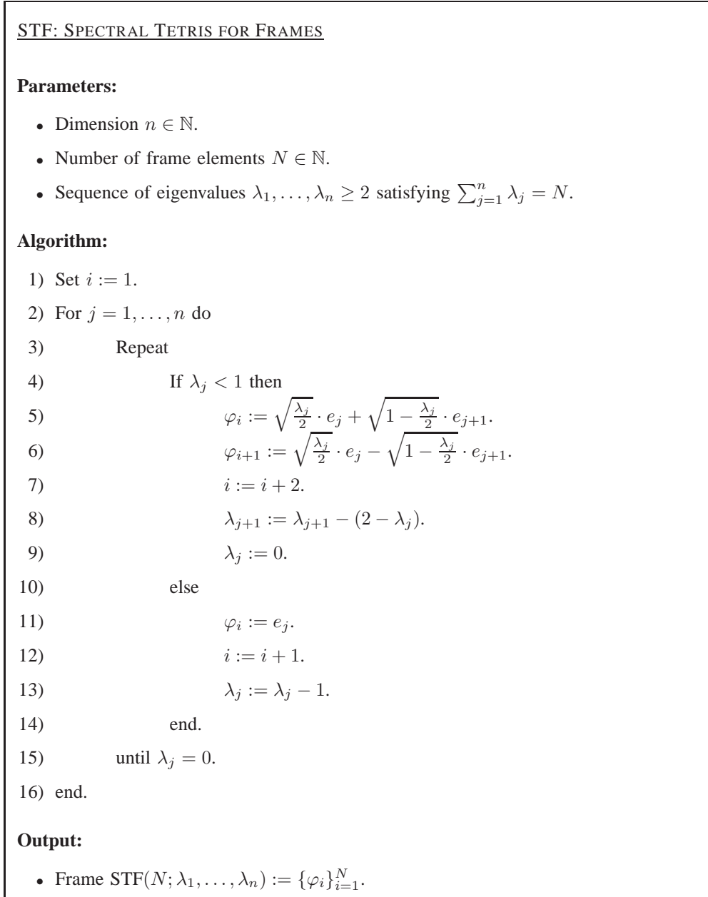
Fig. 1. The Spectral Tetris algorithm for constructing an N -element unit norm frame \text{STF}(N; \lambda_1, \dots, \lambda_n) for \mathbb{R}^n with an associated frame operator having eigenvalues \lambda_1, \dots, \lambda_n .
